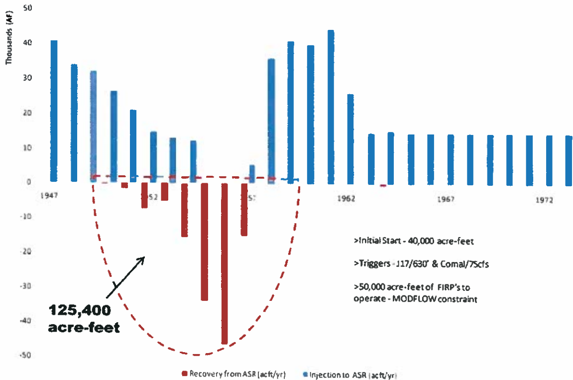
GRAPH 1 LATEST EARIP MODELED HYPOTHETICAL OPERATION (HDR Simulation 1-13-2011)
