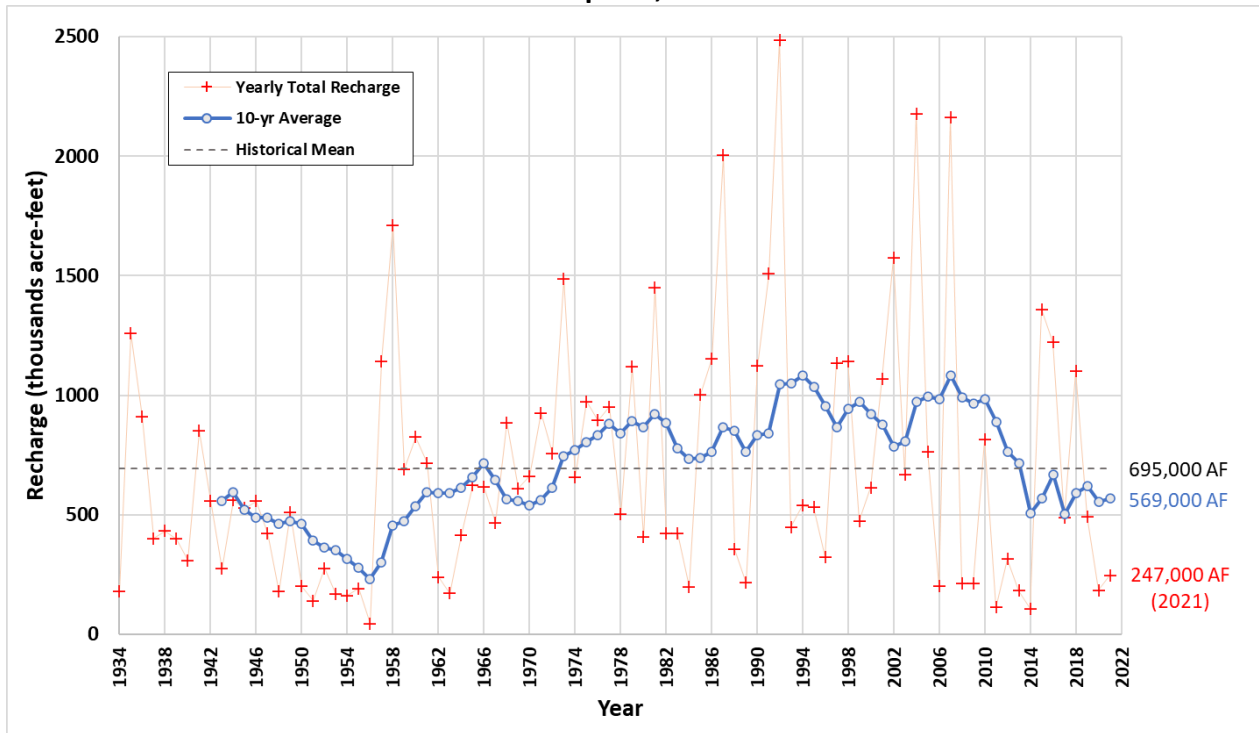
Figure 2. Estimated Annual Recharge for the San Antonio Segment of the Balcones Fault Zone Edwards Aquifer, 1934–2021.
