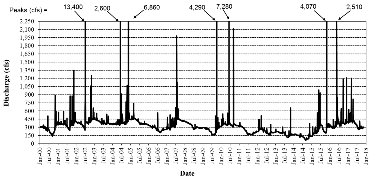
Figure 12. Comal River hydrograph presented as daily discharge over the biological monitoring period.
