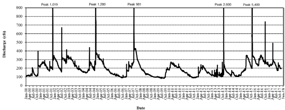
Figure 13. San Marcos River hydrograph presented as daily discharge over the biological monitoring period.
