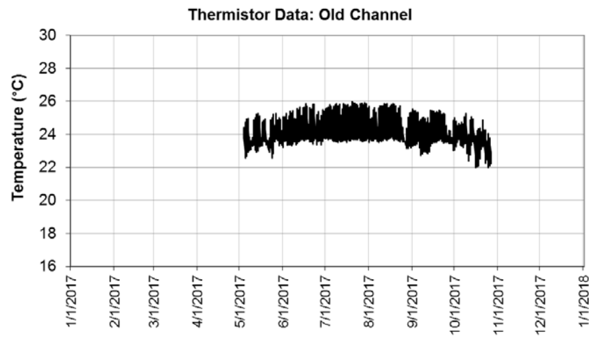
Figure 14. Thermistor data collected during 2017 at four select sites extending upstream to downstream in the Comal System.
