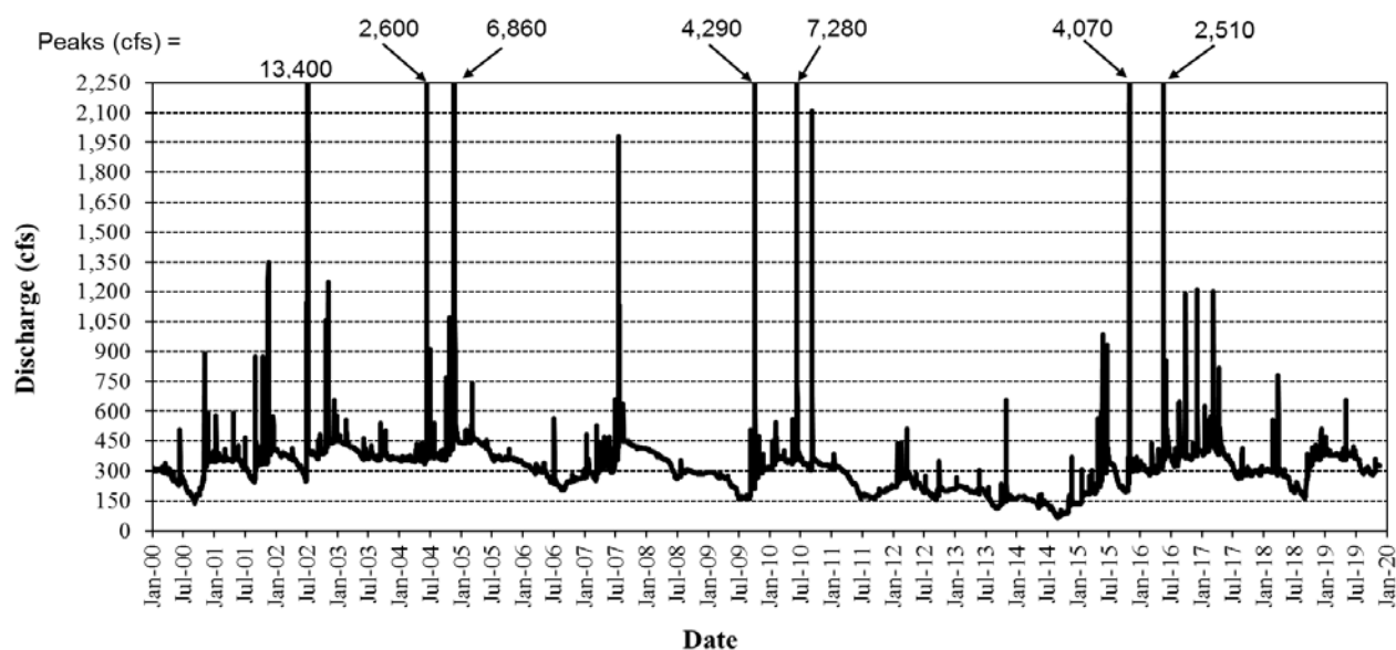
Figure 8. Comal River hydrograph presented as daily discharge over the biological monitoring period.
