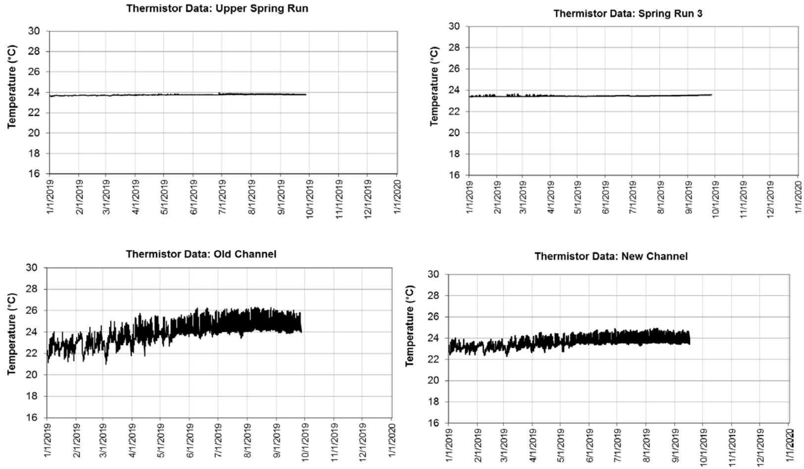
Figure 10. Thermistor data collected during 2019 at four select sites extending upstream to downstream in the Comal System.
