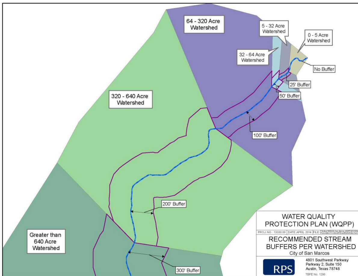
Figure 8-1 Diagram of Recommended Stream Buffers
