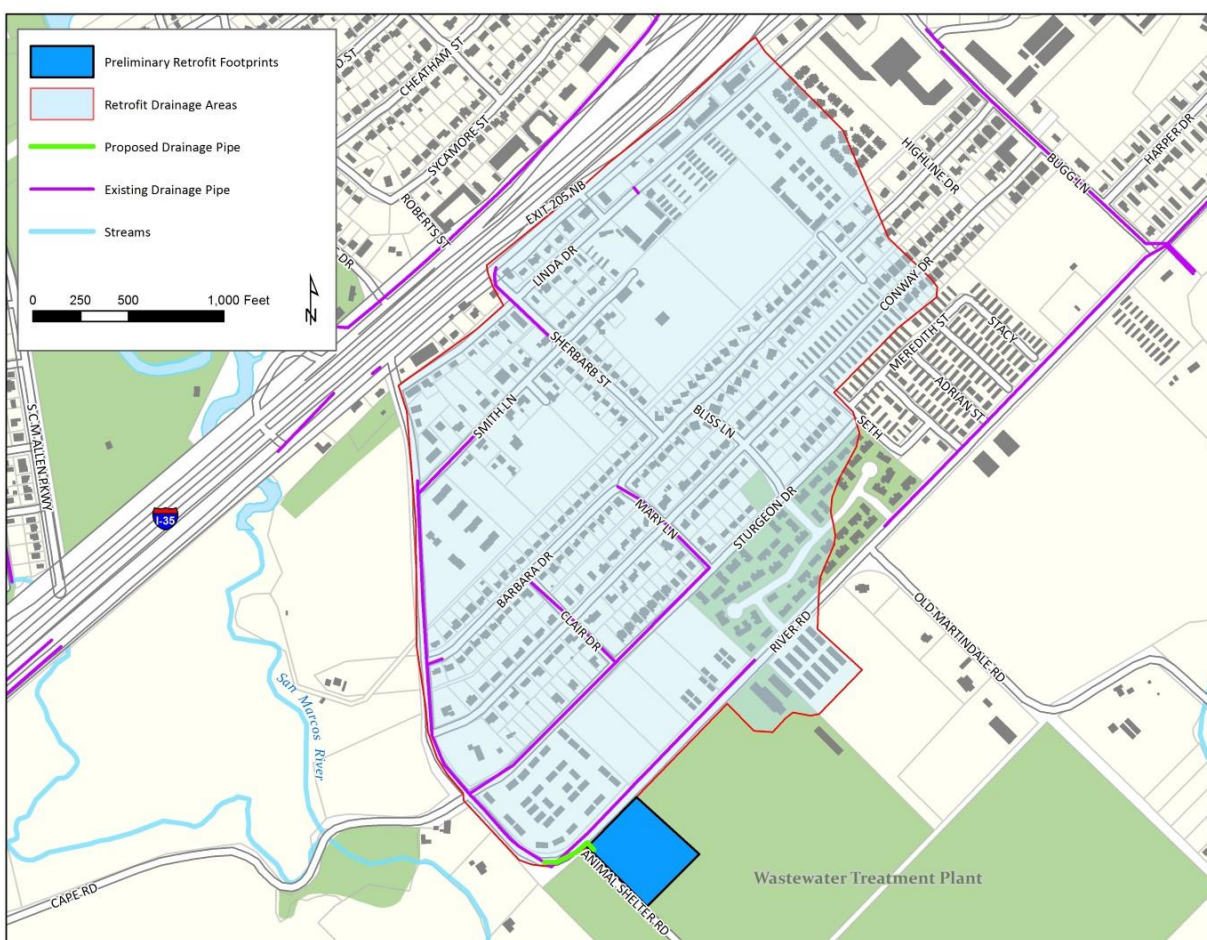
Figure 8-15 Wastewater Treatment Plant Retrofit: Concept Plan
