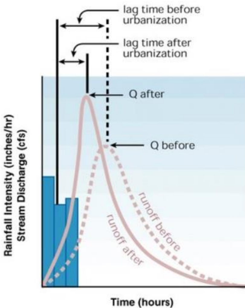
Figure 6-3 Hydrographs Before and After Development
