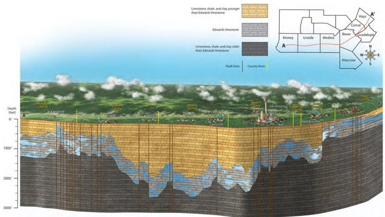
Figure 1-6 Cross-Section through the Edwards Aquifer
