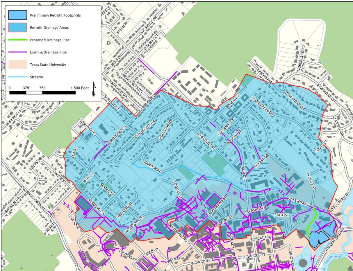
Figure 9-6 Fish Ponds 3: Concept Plan
