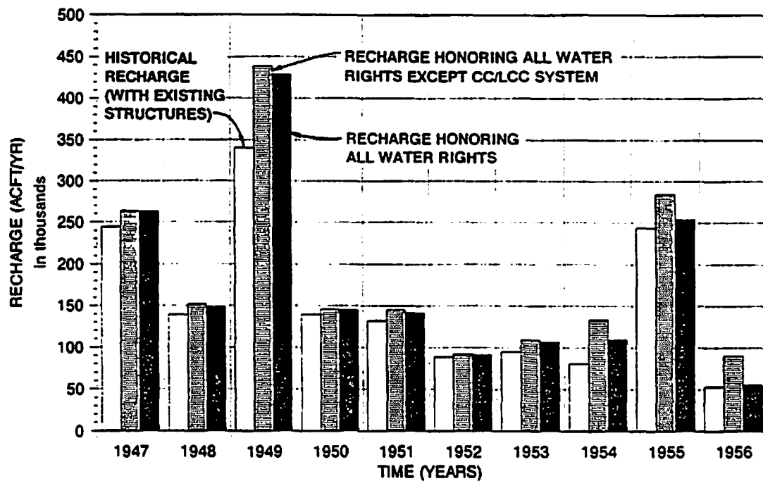
TYPE 1 RECHARGE STRUCTURES
