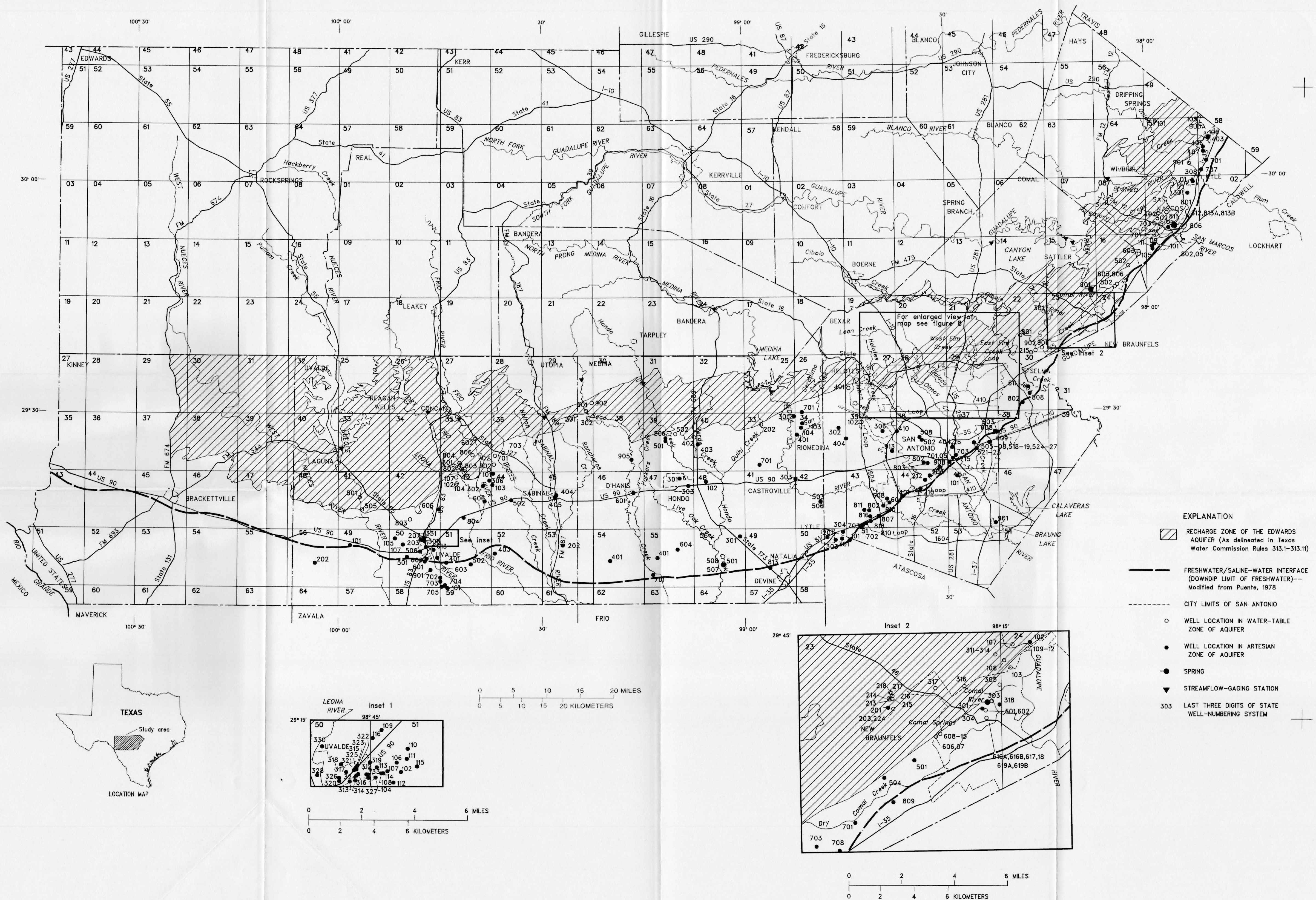
Plate 5.--Location of water-quality data-collection sites--wells, springs, and streams--sampled during 1972-91.
