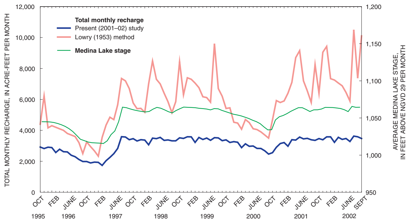
Figure 13. Comparison of monthly recharge to the Edwards aquifer in the study area during October 1995–September 2002, as estimated by the present (2001–02) study and computed with the Lowry (1953) method.
