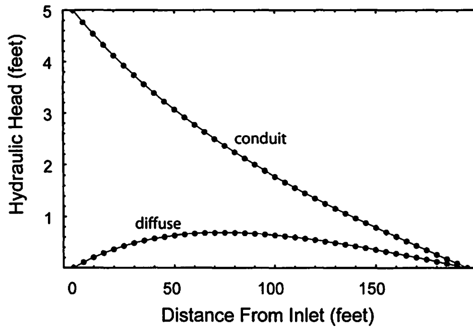
Figure 2.3 Results of the dual-conductivity validation test at t = 20 minutes. The benchmark results are shown as solid lines and the DCM results as individual data points. The upper set represents the hydraulic head in the conduit system and the lower set represents the hydraulic head in the matrix system.
