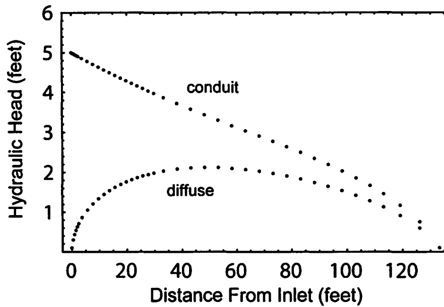
Figure 2.5 Steady-state results for the unconfined flow validation test (Test 2a). This simulation was used to verify that water balance is properly maintained in the DCM package.
