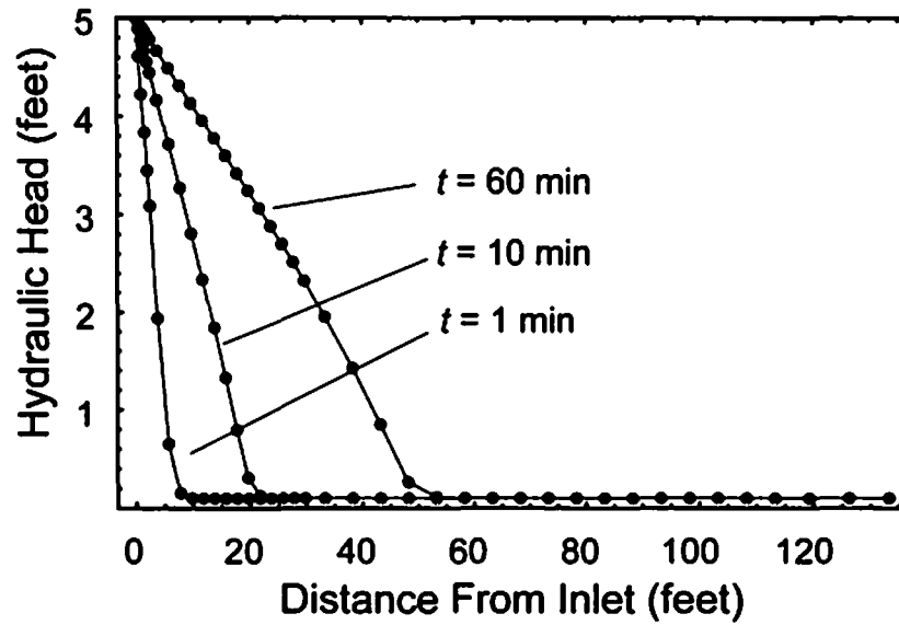
Figure 2.4 Results of the unconfined flow validation test (Test 2) at t = 1 , 10, and 60 minutes. The hydraulic heads in the conduit as calculated by the standard MODFLOW LPF package are shown as solid lines and the DCM results as individual data points.
