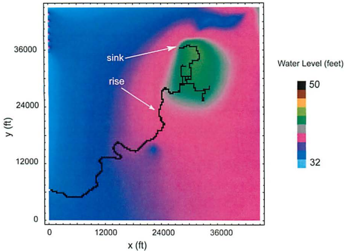
Figure 4.16 Case III. Contour map of the transient head distribution during peak discharge in the diffuse continuum with a reduction in the matrix/conduit exchange parameter \alpha_0 from 1.0 to 0.01. [Data are feet above NGVD29.]
